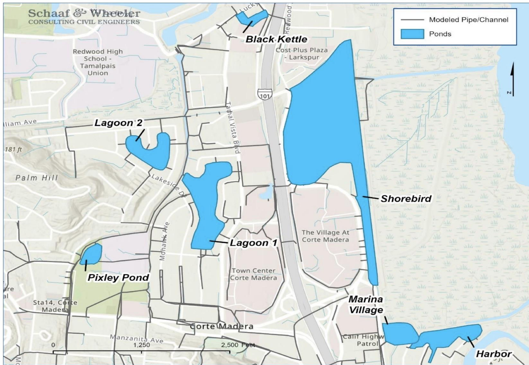
Figure 3-2: Modeled Storage/Detention Basin Locations
