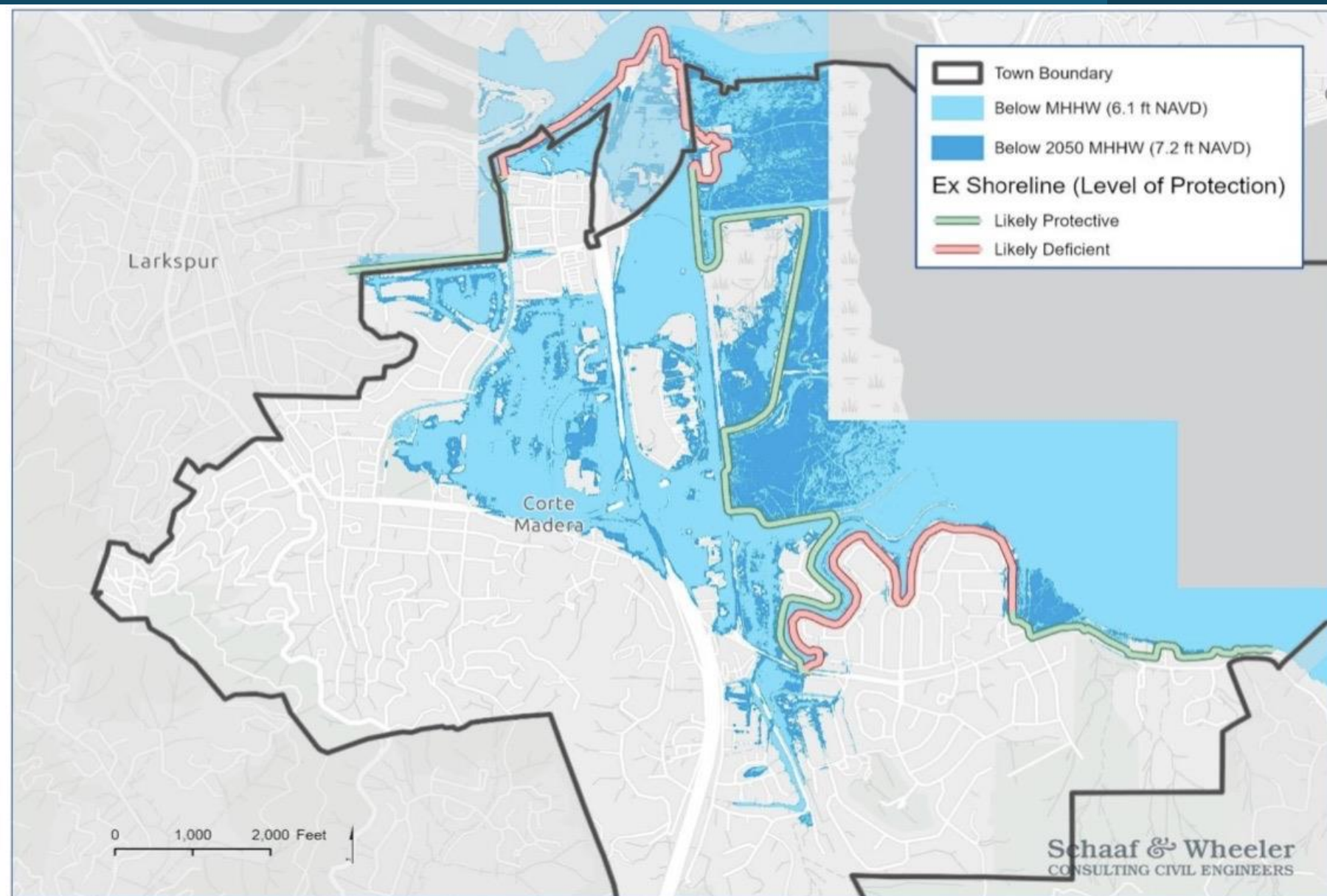
Figure 4-6: Areas Below MHHW Level (2050 High Emissions SLR) and Level of Protection Provided by Existing Shoreline Elevations
