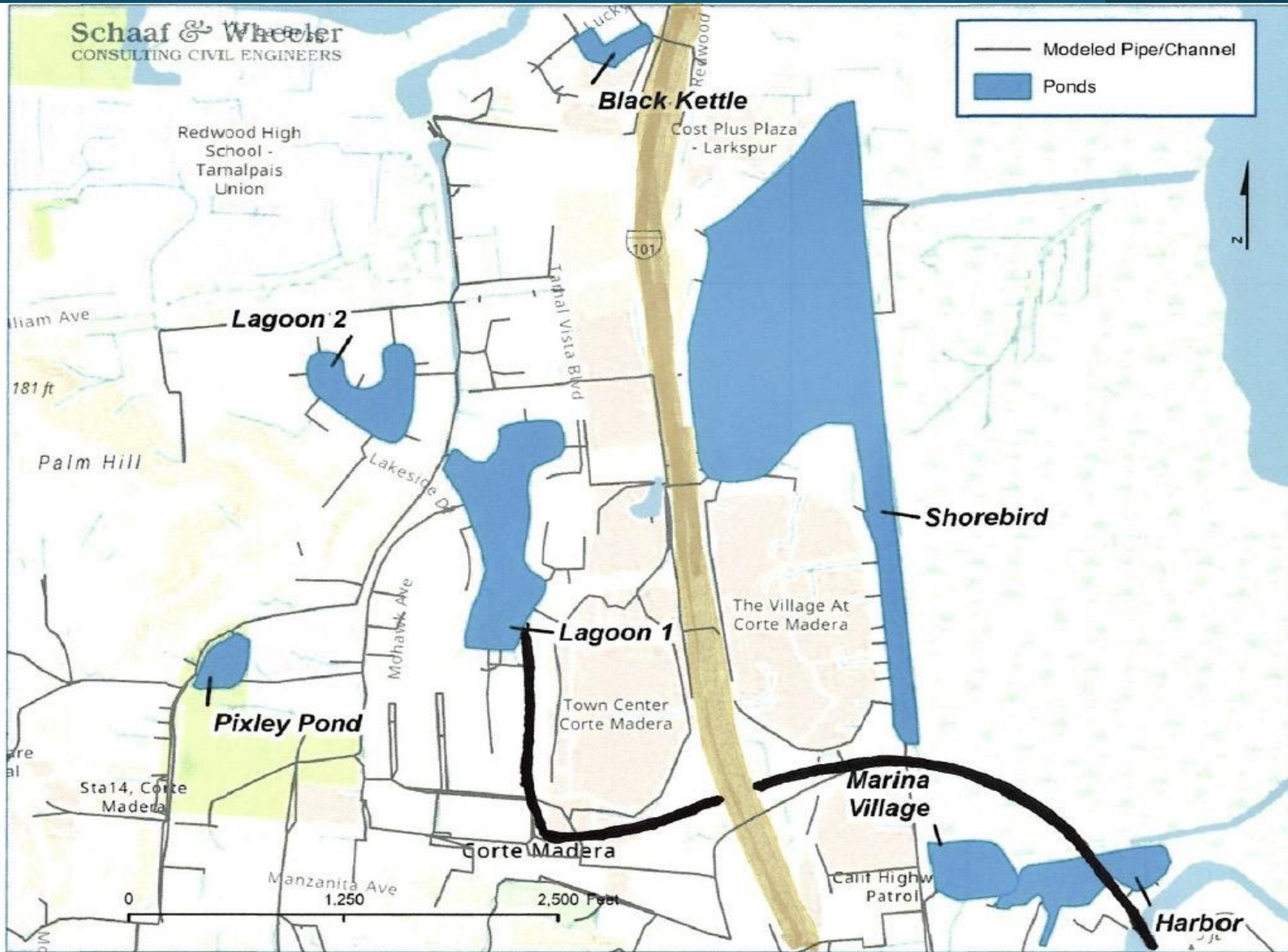
Figure 3-2: Modeled Storage/Detention Basin Locations
