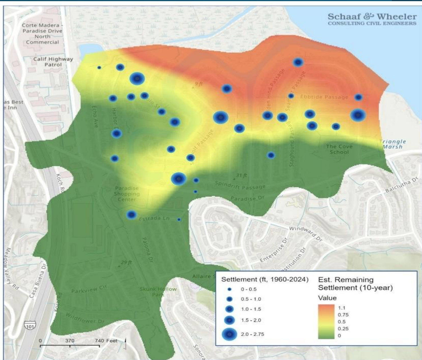
Figure 5-23: Expected 10-year Settlement Based on Bay Mud Consolidation on a 10-year Time Horizon Surrounding San Clemente Creek
